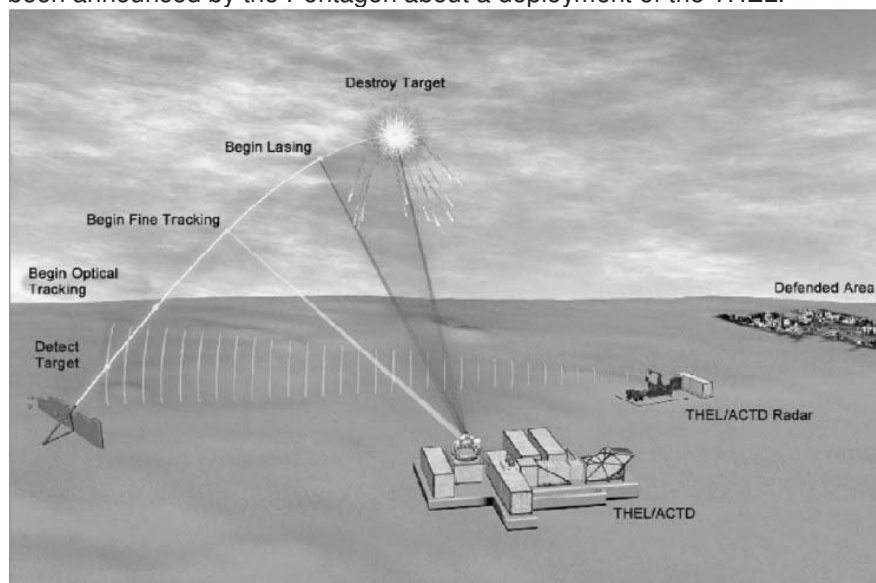
Figure 3: Progress of a THEL Engagement. Source: Schwartz et al. (as in n. 29).
